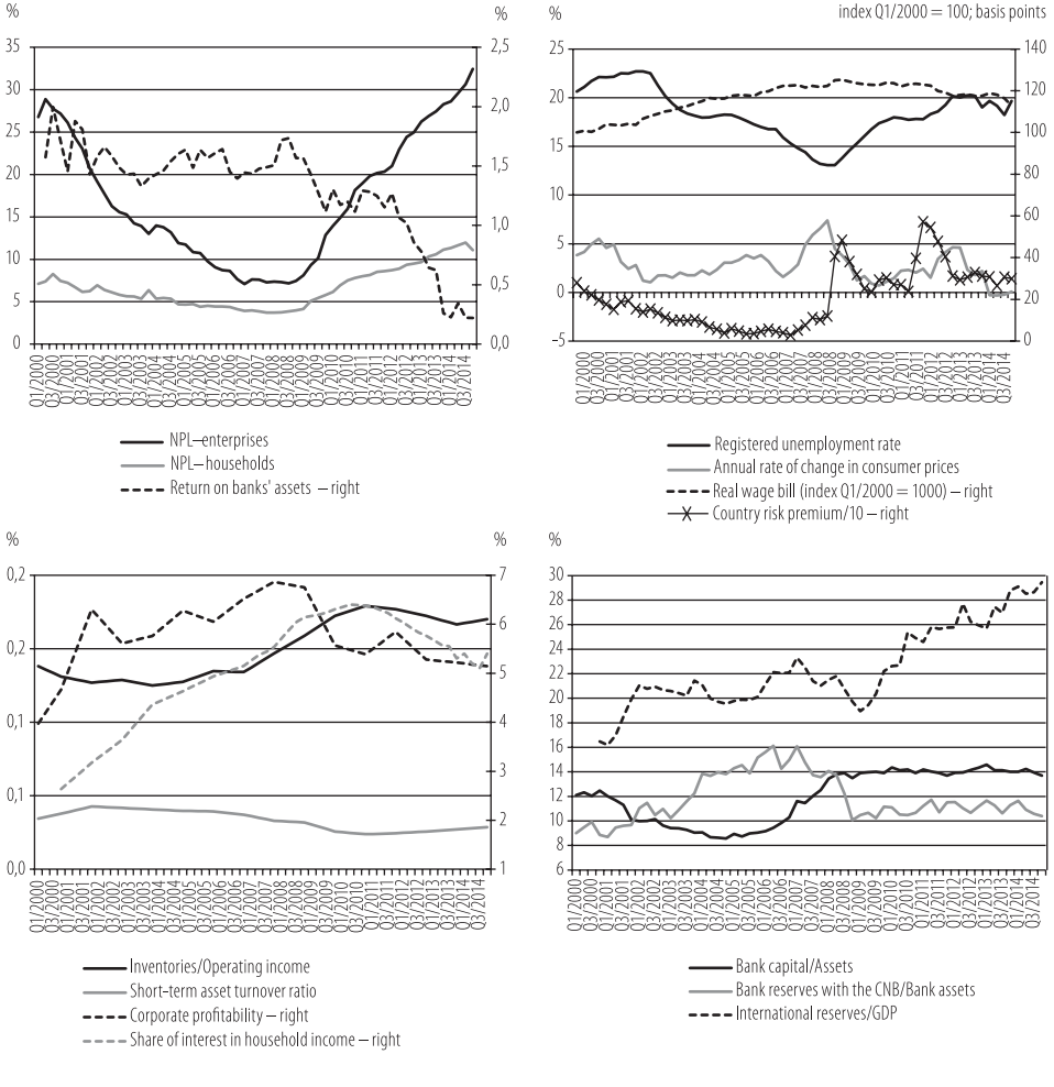
Figure 4: Developments in the components of the systemic risk materialisation index
