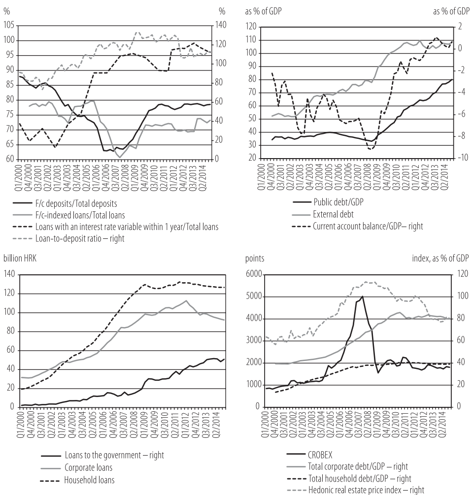
Figure 1: Developments in components of the systemic risk accumulation index
