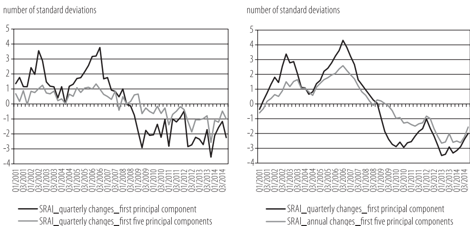
Figure 2: Systemic risk accumulation indicators
