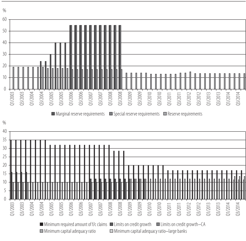
Figure 3: Changes in the most important monetary policy measures from 2003 until end-2014
