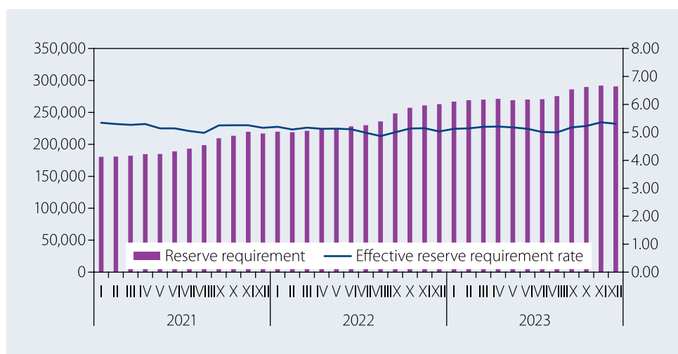
Graph 7 – Allocated reserve requirement in thousand euros (left-hand scale), effective reserve requirement rate, in % (right-hand scale), January 2021 - December 2023, end-month balance
