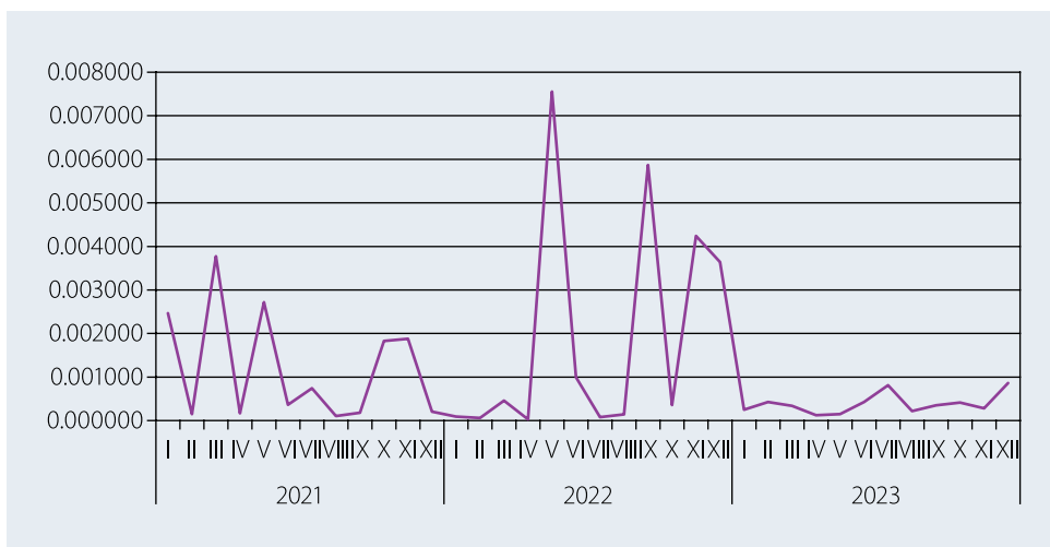
Graph 9 – Asset turnover ratio, January 2021 - December 2023, end-month balance
