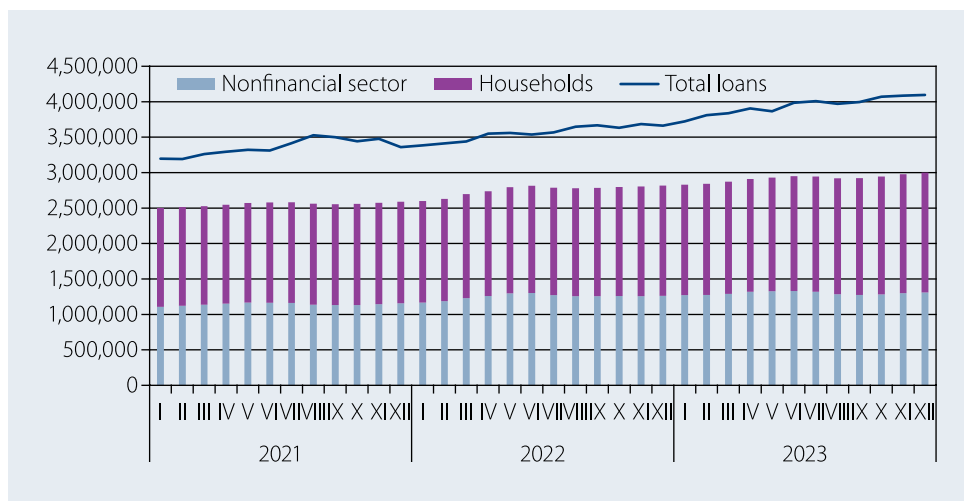
Graph 5 – Loans to households, nonfinancial sector, and total banking loans, in thousand euros, January 2021 - December 2023, end-month balance
