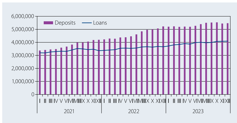
Graph 4 – Loans and deposits, in thousand euros, January 2021 - December 2023, end-month balance
